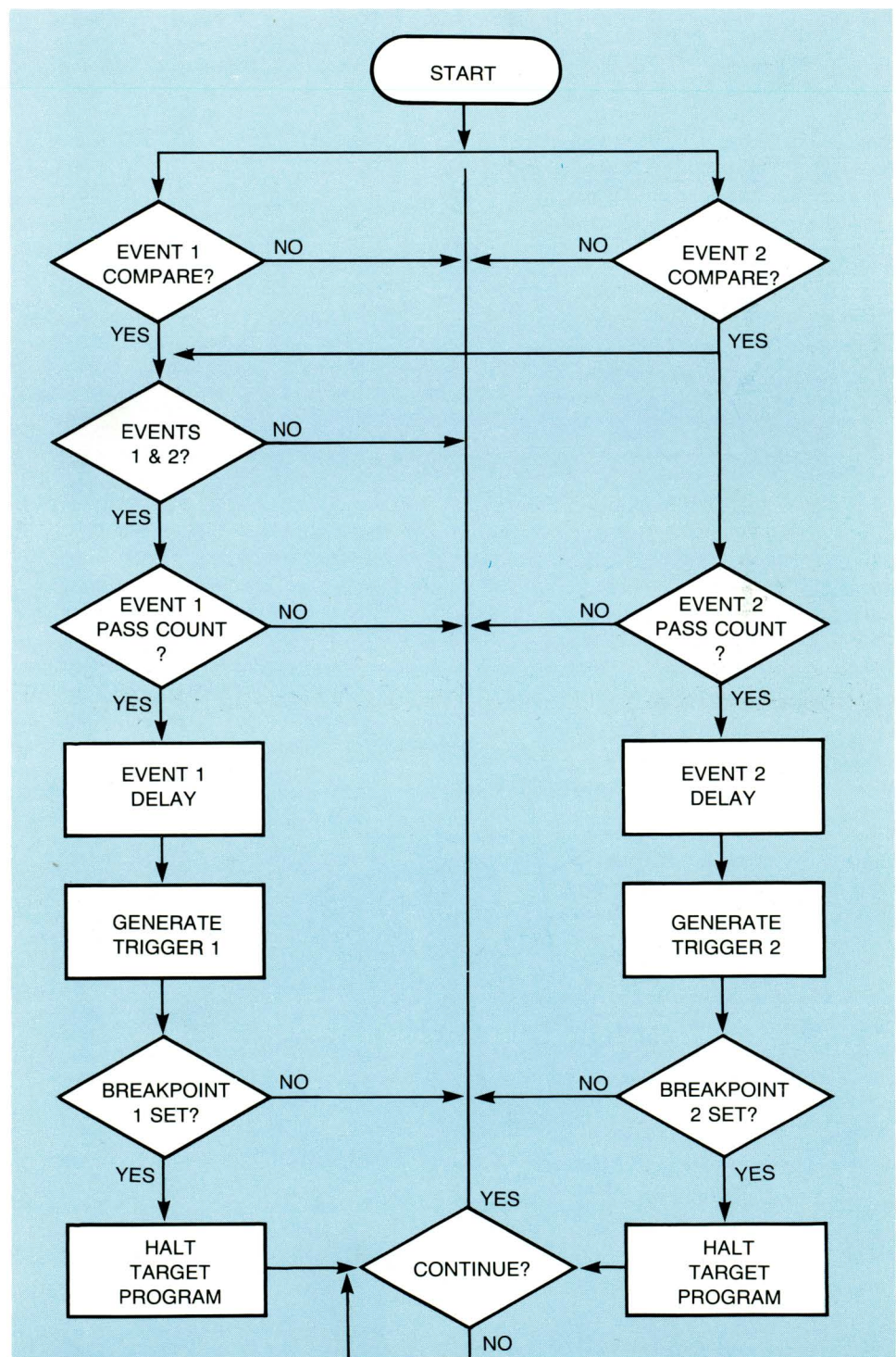
Figure 7. Limit Mode.
